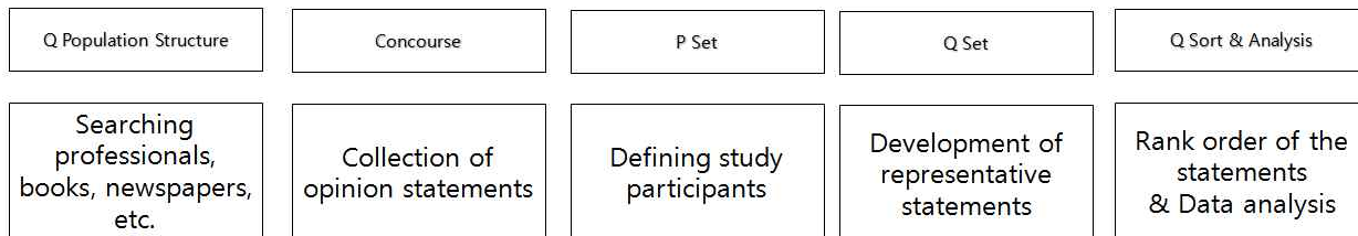
Fig. 1. Research flow.
